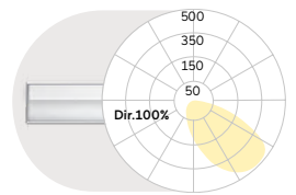
Wallwasher | Direct
