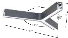
Y3-Junction
