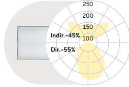
Wallwasher | Direct-Indirect
