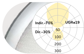
Microprismatic | Direct-Indirect
