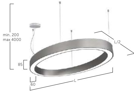
Parallel Suspension
