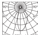
Luminous flux luminaire 2560 lm
