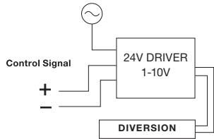
Driver Option 2 (1-10V)
