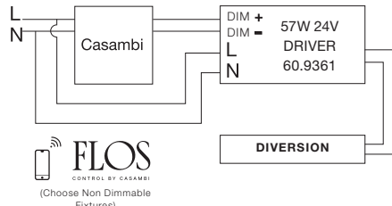
Driver Option 3 Casambi Interface
