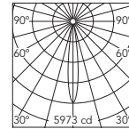
Luminous flux luminaire 418 lm
