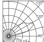
Luminous flux luminaire 2676 lm
