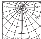
Luminous flux luminaire 687 lm
